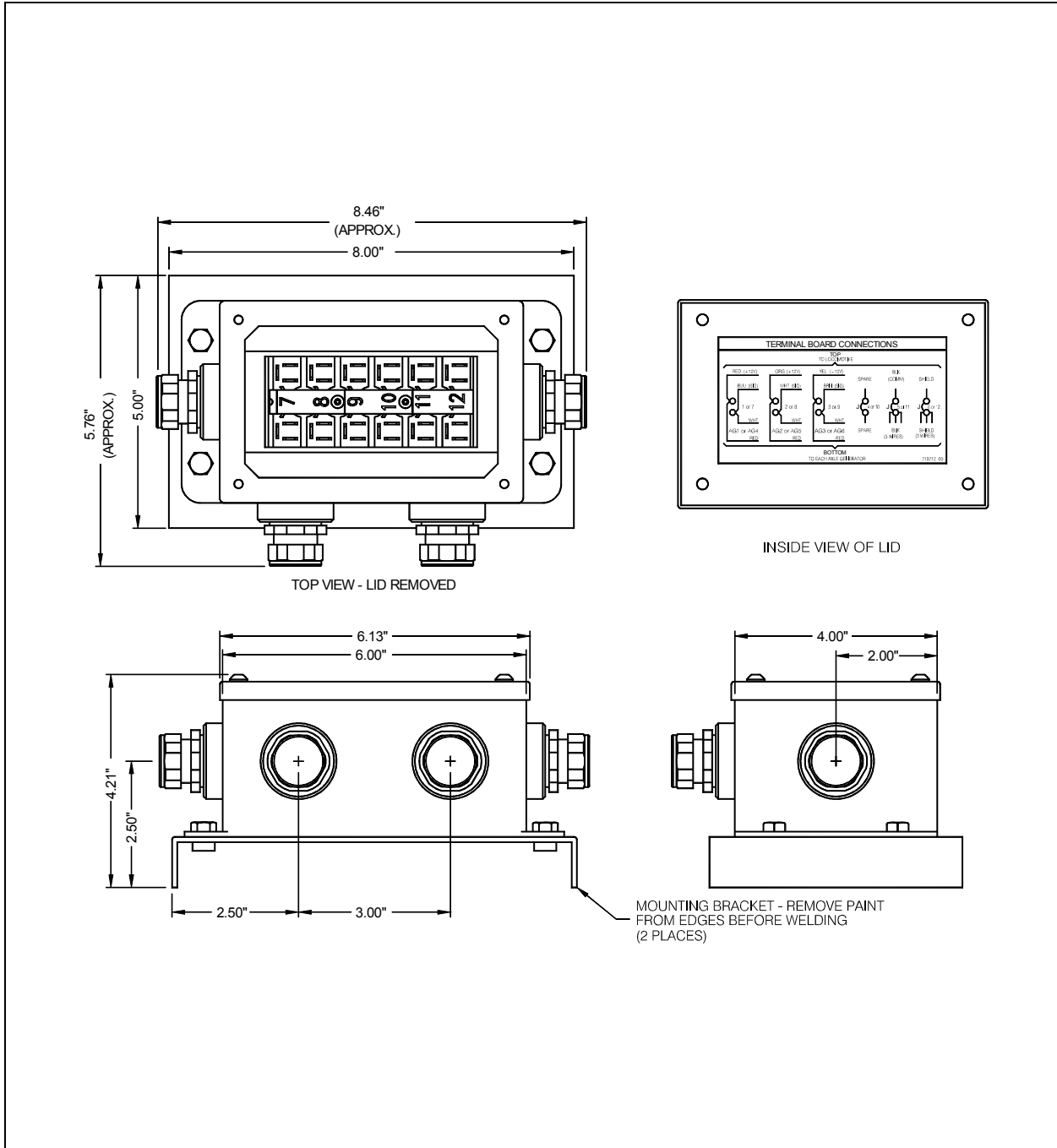
Figure 1. Axle Generator Junction Box, Positions 7-12 application
