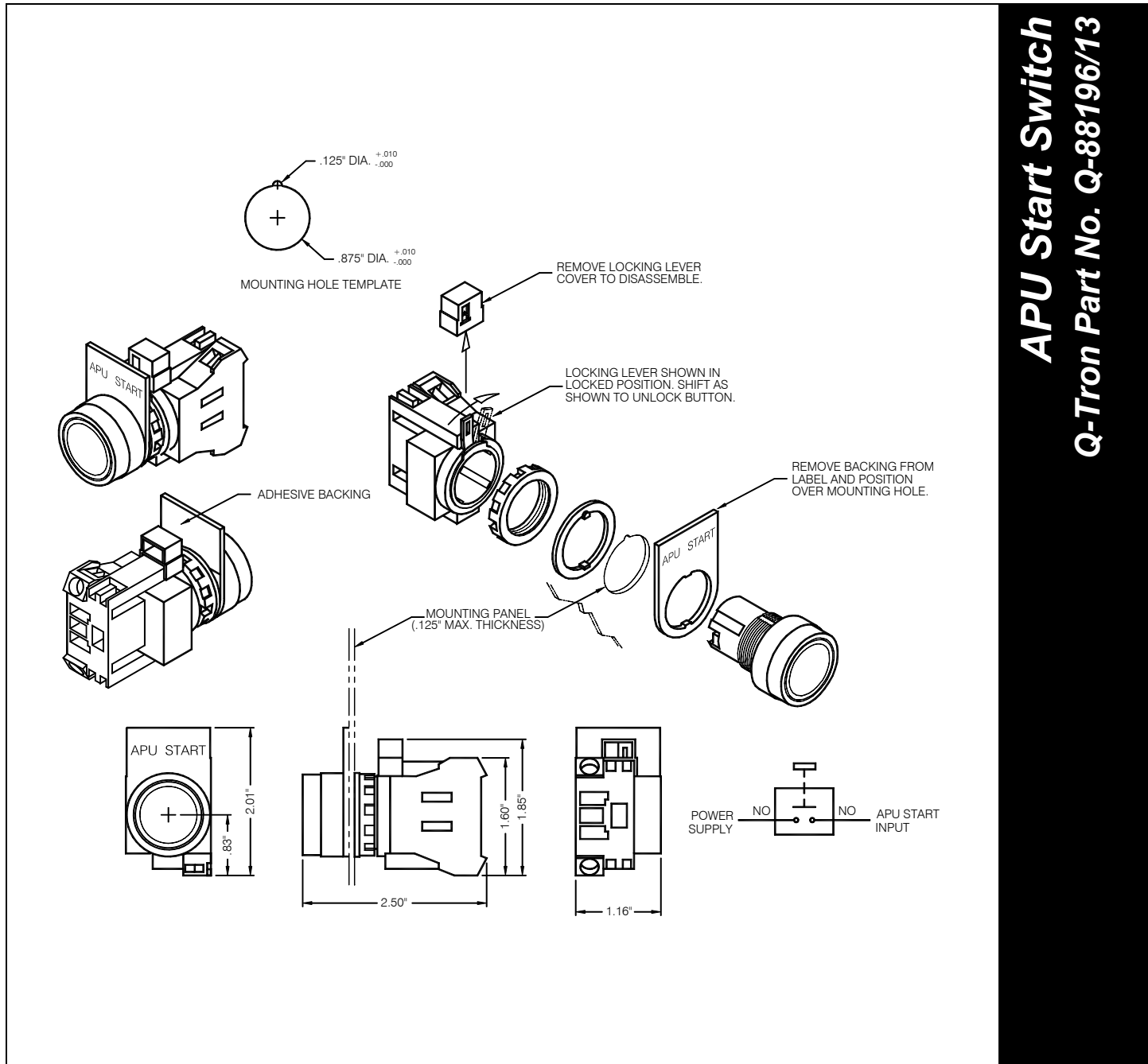
Figure 1. APU Start Switch application
